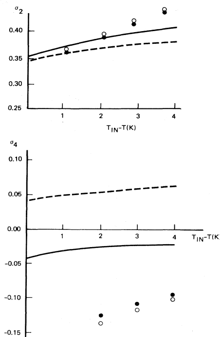
FIG. 1. Order parameters \sigma_2 and \sigma_4 as functions of temperature. \circ , Ref. 12; \bullet , Ref. 13; ---, Ref. 8 (theoretical curve without anisotropic steric potentials); —, present work.
